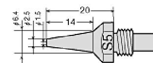
*TP-100N-S5
