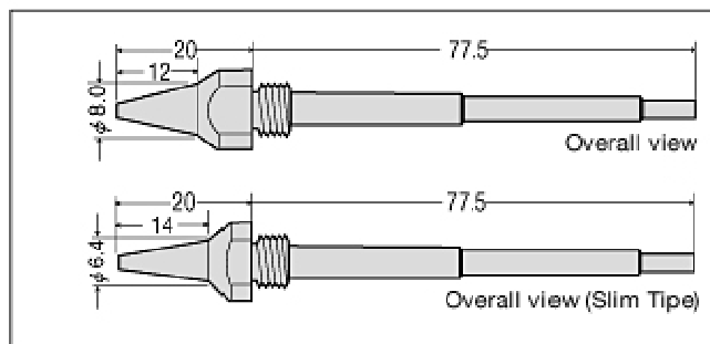
*TP-100N-S1
